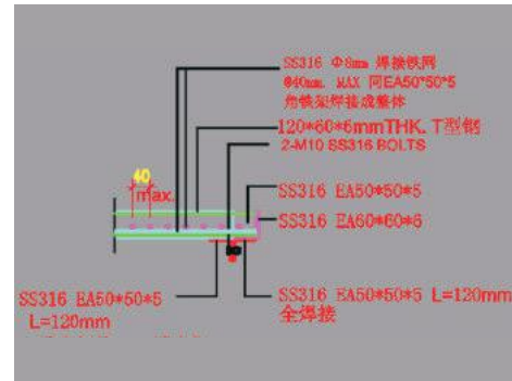
● 安装示意 Installation drawing
